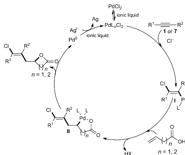
Scheme 6. Plausible reaction mechanism.
