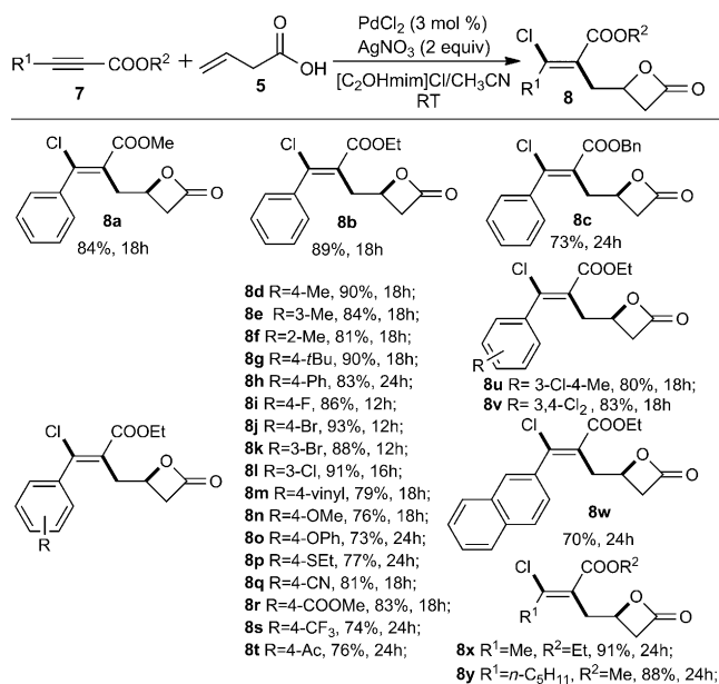
Scheme 4. Cascade annulation of alkynoates with 5 in [\text{C}_2\text{OHmim}]\text{Cl} . Reaction conditions: 7 (0.25 mmol), 5 (0.30 mmol), \text{PdCl}_2 (3 mol %), \text{AgNO}_3 (0.5 mmol), [\text{C}_2\text{OHmim}]\text{Cl} (0.5 mL), and \text{CH}_3\text{CN} (0.1 mL) at room temperature.
